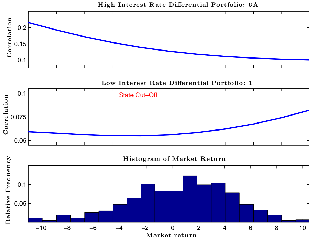
Figure 3: Kernel-Smoothed Conditional Correlation
