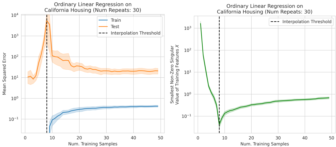
Figure 5: Double Descent in Ordinary Linear Regression on California Housing Dataset.
