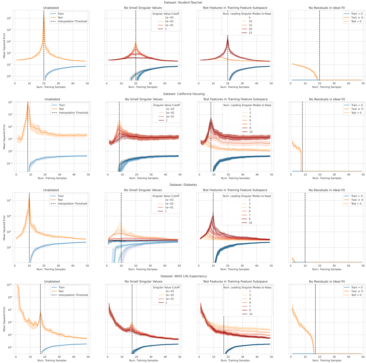
Figure 7: Double descent will not occur if any of the three critical quantities are absent. We demonstrate this via ablations (Sec. 6). Left to Right: Double descent appears in ordinary linear regression. Removing small singular values in the training features X prevents double descent. Preventing the test features \vec{x}_{test} from varying in the trailing singular modes of the training features X prevents double descent. Ensuring that the optimal model in the model class has zero residual prediction errors E prevents double descent. Top to Bottom: Synthetic data generated in a Student-Teacher framework, California Housing dataset, Diabetes dataset, WHO Life Expectancy dataset
