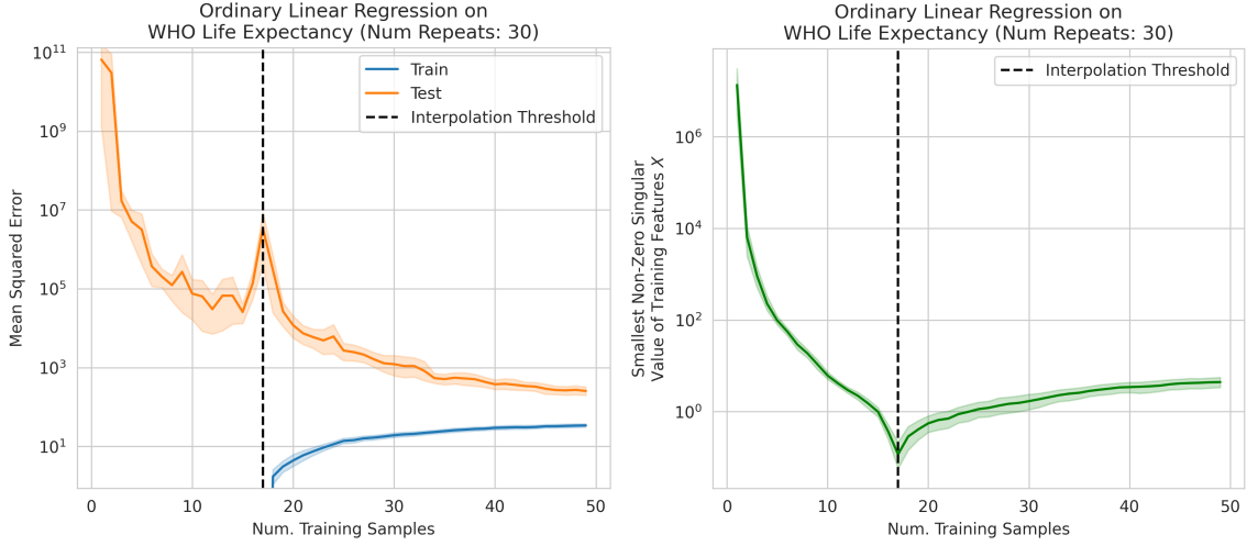
Figure 3: Left: Double descent occurs in ordinary linear regression on the World Health Organization’s Life Expectancy dataset. Right: Double descent occurs when three quantities simultaneously grow extreme. One of the three is small-but-nonzero singular values in the training features X . The smallest non-zero singular value of X (probabilistically) obtains its lowest value when the number of parameters P equals the number of data N (the interpolation threshold ), approaching from either the overparameterized regime ( P > N ; left) or the underparameterized regime ( P < N ; right).
