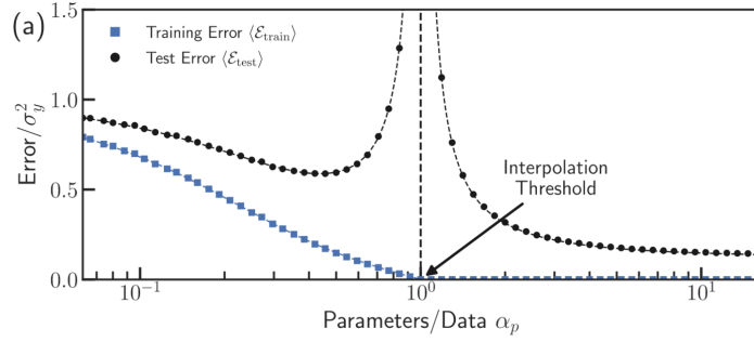
Figure 1: Double descent: test error falls, rises, then falls as a ratio of parameters to data. Fig. 3A from [18].
