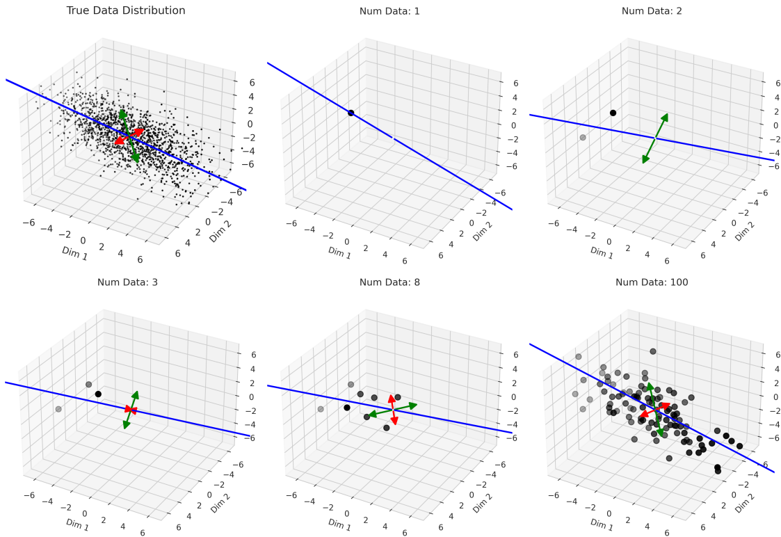
Figure 4: Geometric intuition for why the smallest non-zero singular value reaches its lowest value when approaching the interpolation threshold. As one nears the interpolation threshold (here, D = P = N = 3 ), N training data are unlikely to vary substantially in P orthogonal directions, meaning at least one orthogonal direction is likely to have small variance. If fewer data are observed, then the trailing directions have exactly zero variance, and if more data are observed, then the additional data reveal variance along these trailing directions.
