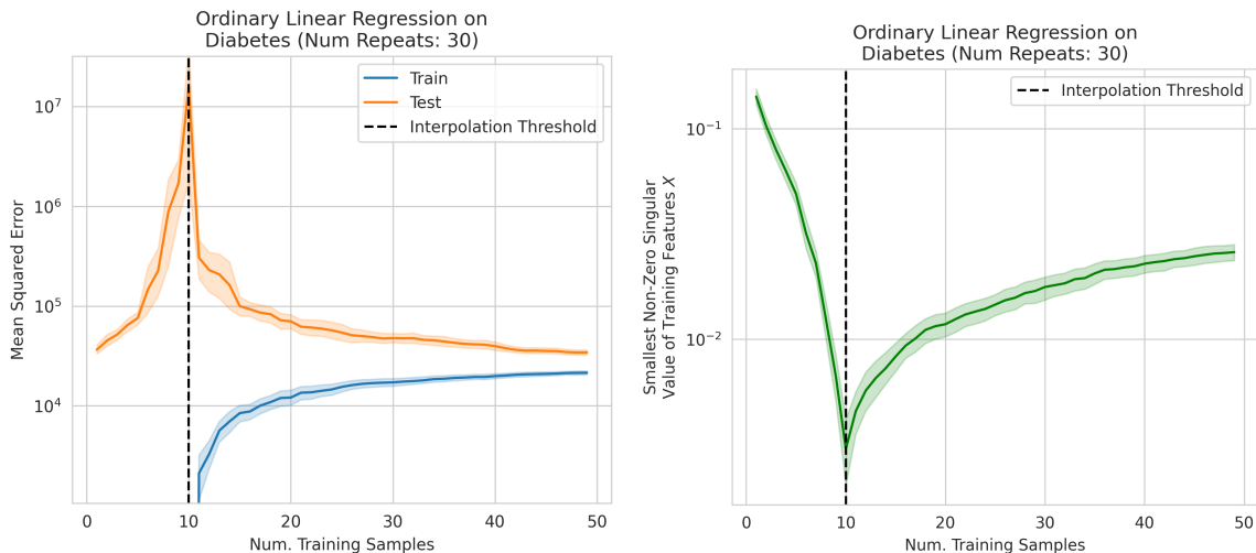
Figure 6: Double Descent in Ordinary Linear Regression on Diabetes Dataset.
